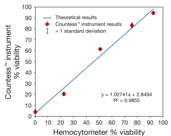
Countess™ Automated Cell Counter vs. hemocytometer.
